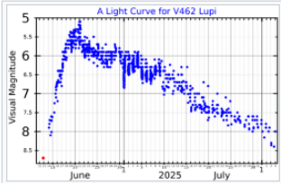
A visual band light curve for V462 Lupi, plotted from AAVSO [5] and ASAS-SN [1] data (red point)
