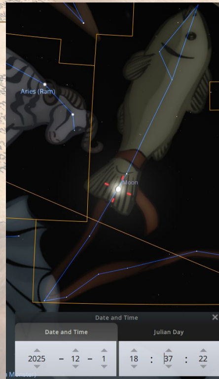
PREDICTED
